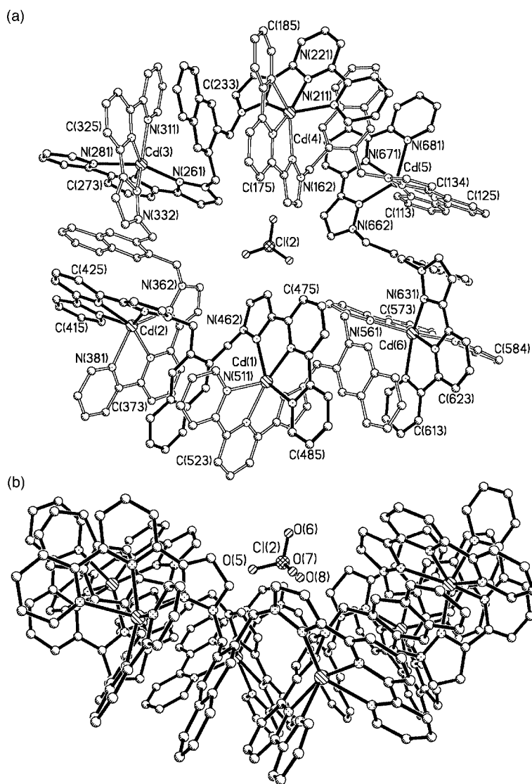
Figure 6. Two views of the structure of the complex cation of [\text{Cd}_6(\text{L}^{\text{naph}})_6](\text{ClO}_4)_{12} : (a) a face-on view, with the ligands shaded alternately dark and light for clarity, emphasising the cyclic helical structure and the encapsulated anion in the centre; (b) an edge-on view showing the shallow bowl shape of the cation.
