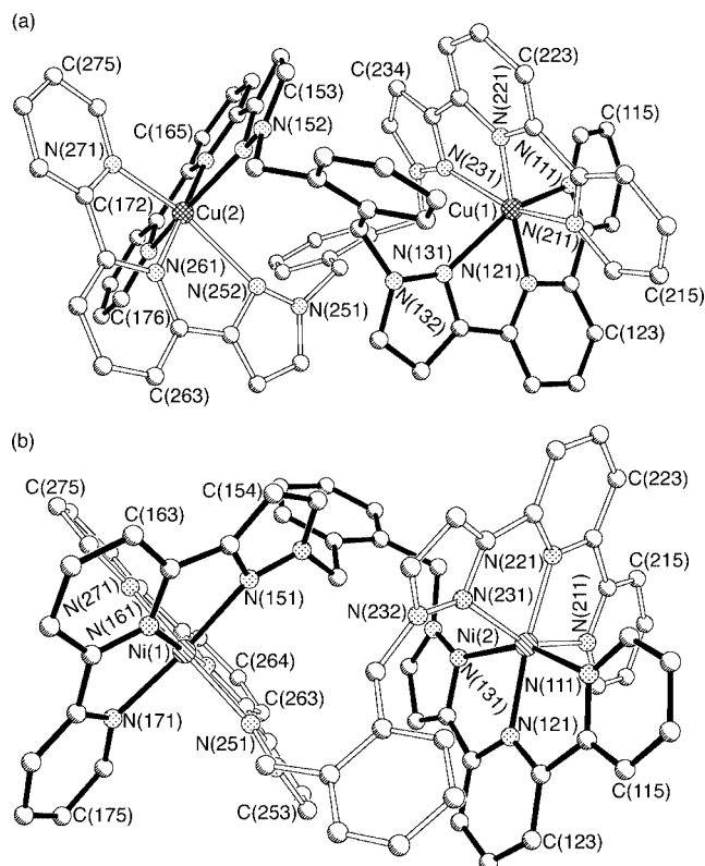
Figure 2. Structures of the double helical complex cations of (a) [\text{Cu}_2(\text{L}^{\text{Ph}})_2][\text{ClO}_4]_4 \cdot 2\text{MeCN} \cdot 0.5\text{H}_2\text{O} and (b) [\text{Ni}_2(\text{L}^{\text{Ph}})_2][\text{ClO}_4]_4 \cdot \text{MeCN} , with the ligands shaded differently for clarity.
