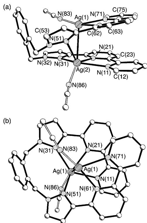
Figure 3. Structure of the complex cation of [\text{Ag}_2(\text{L}^{\text{Ph}})(\text{MeCN})_2][\text{BF}_4]_2 (MeCN ligands are shown shaded differently for clarity).
