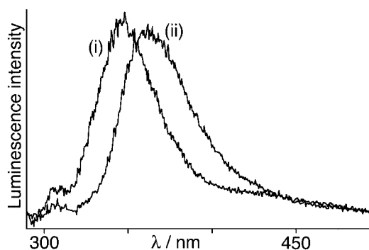
Figure 8. Luminescence spectra of solutions of (i) [\text{Ag}_3(L^{\text{naph}})_2](\text{BF}_4)_3 and (ii) [\text{Cd}_6(L^{\text{naph}})_6](\text{ClO}_4)_{12} in MeCN, concentration ca. 10^{-6} M; the solutions had the same optical density at the excitation wavelength.
