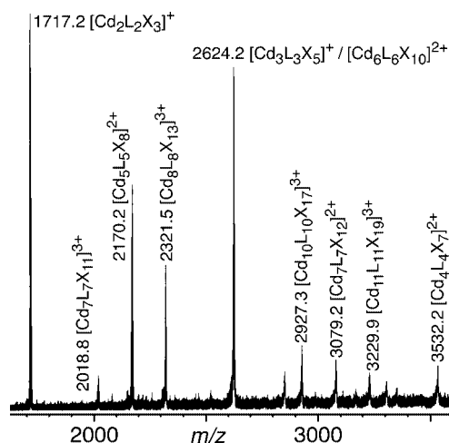
Figure 7. Part of the electrospray mass spectrum of redissolved crystals of [Cd 6 (L naph ) 6 ](ClO 4 ) 12 , showing the presence of a range of cyclic oligomers in solution.
