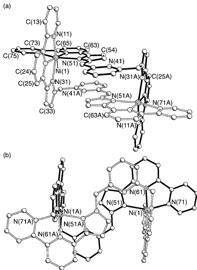
Figure 4. Two views of the complex cations of the mesocate [\text{Ni}_2(\text{L}^{\text{Py}})_2][\text{BF}_4]_4 \cdot 2\text{MeNO}_2 , with the ligands shaded differently for clarity.
