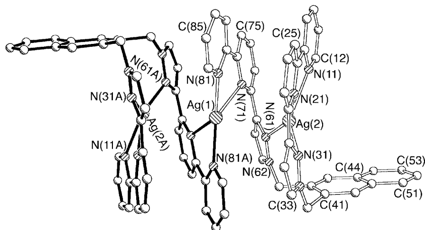
Figure 5. Structure of the complex cation of [\text{Ag}_3(\text{L}^{\text{naph}})_2](\text{BF}_4)_3 \cdot 2\text{MeCN} , with the two ligands shaded differently for clarity.
